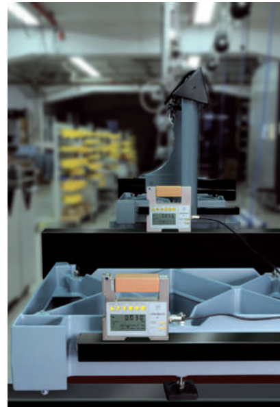
When 2 CLINOBEVEL 2 are connected, one of the instruments becomes the reference
